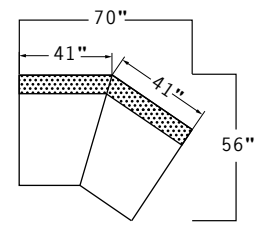
#70 ARMLESS ANGLE 70"
